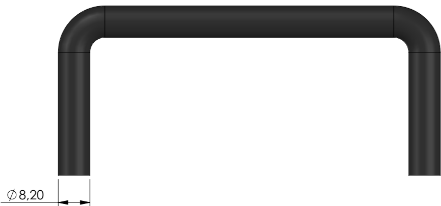
ROUNDRACK3.9
